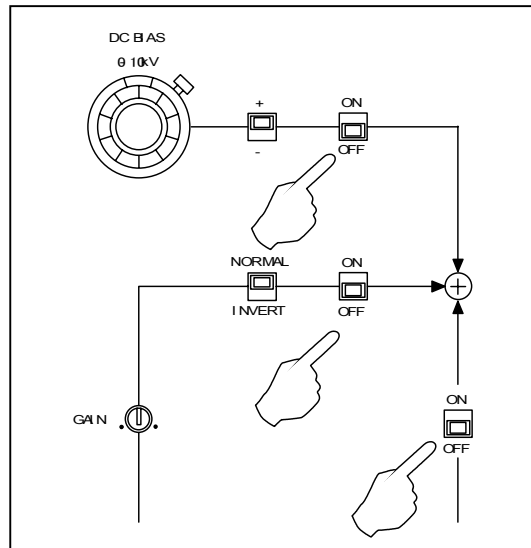
Figure4-36. Switch settings
