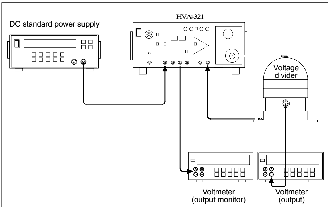
Figure7-2. Check method of constant voltage mode
