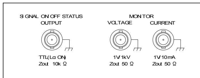
Figure3-15. Monitor output
