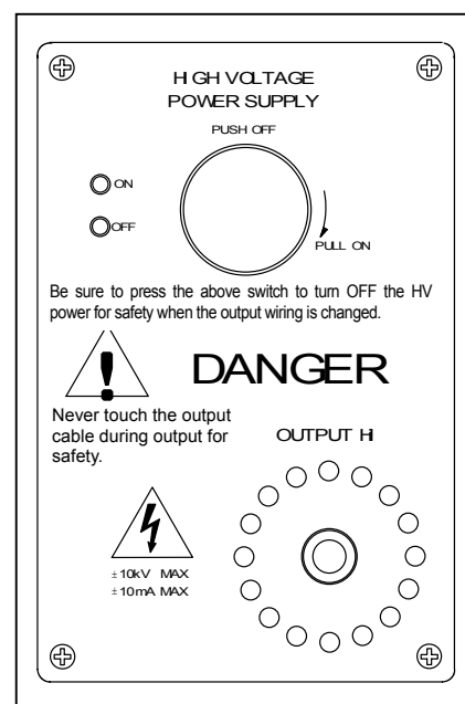
Figure3-12. Output area
