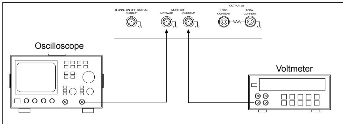
Figure4-11. Connection of monitor
