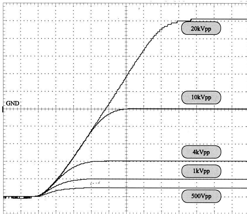
Figure5-16. Step response in constant voltage mode
