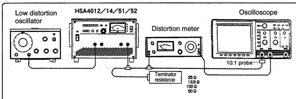
Figure 5-4 Measuring Sine Wave Distortion Rate
