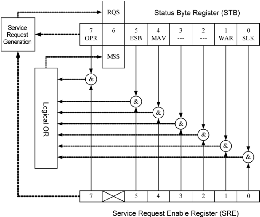
Figure 2.1 Status Byte Register and Service Request Enable Register
