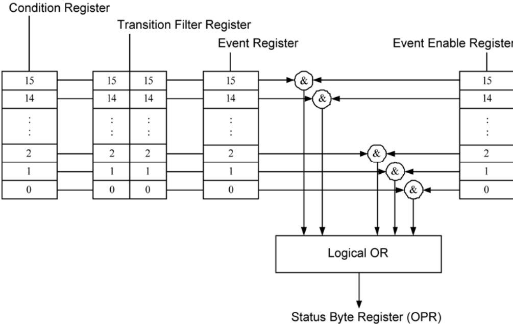
Figure 2.4 Warning Condition Register Group
