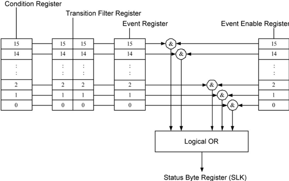
Figure 2.5 System Lock Condition Register Group
