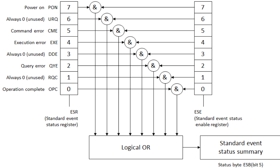
Figure 6-2 Standard event status structure
